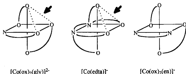
Chart 2. [Co(ox) 2 (gly)] 2- and [Co(edta)] - having the unhindered pseudo -C 3 carboxylate face and [Co(ox) 2 (en)] - having no such a carboxylate face.
